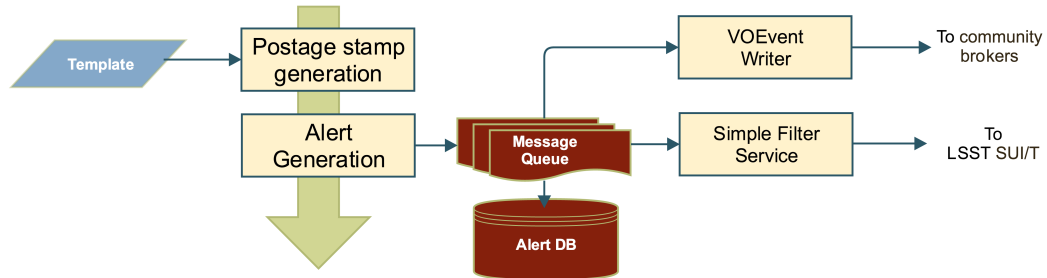
FIGURE 6: Distribution of alerts from the nightly processing: generation of postage stamps around each detected DIAObject, distribution of the DIAObjects as VOEvents, simple filtering of the event stream, and persistence of the events in a database.
