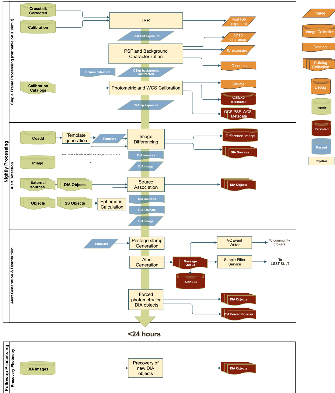
FIGURE 3: The alert production flow of data through the processing pipelines (single frame processing, alert generation, alert distribution, precovery photometry)
