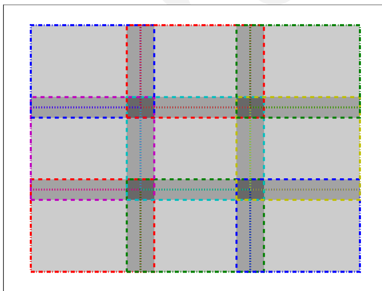
FIGURE 12: Patch boundaries and overlaps regions for a single tract with 3 \times 3 patches. Different colors represent different patches; dashed lines show outer patch regions and dotted lines show inner patch regions. Light gray regions are processed as part of only one patch, medium regions as part of two, and dark regions as part of four.
