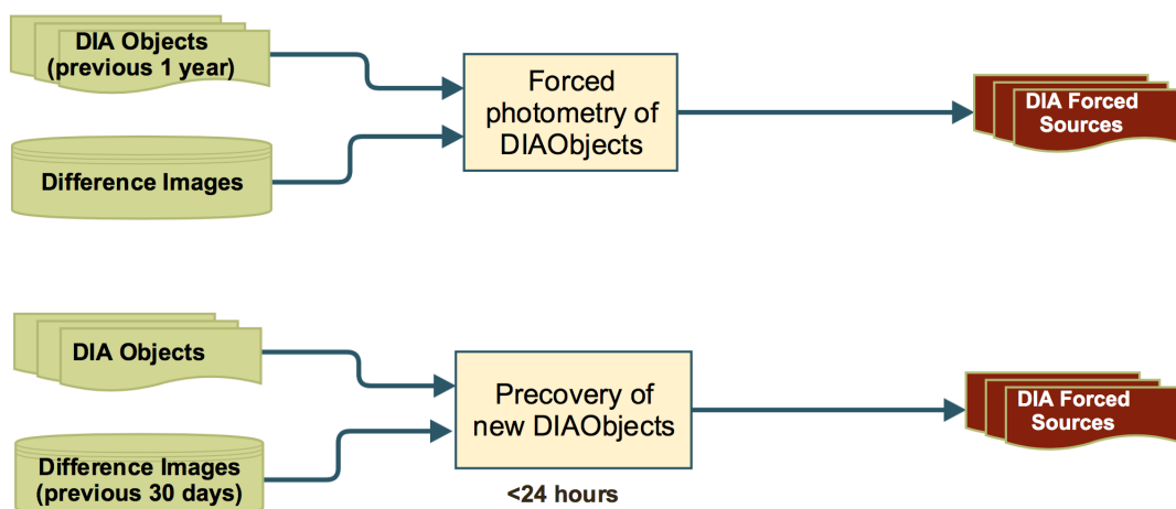
FIGURE 7: Forced photometry for DIAObjects: forced photometry on a night's DiffExp for all DIAObjects that have detected DIASources within the last year, precorecovery photometry for the previous 30 days of DiffExps for new DIAObjects
