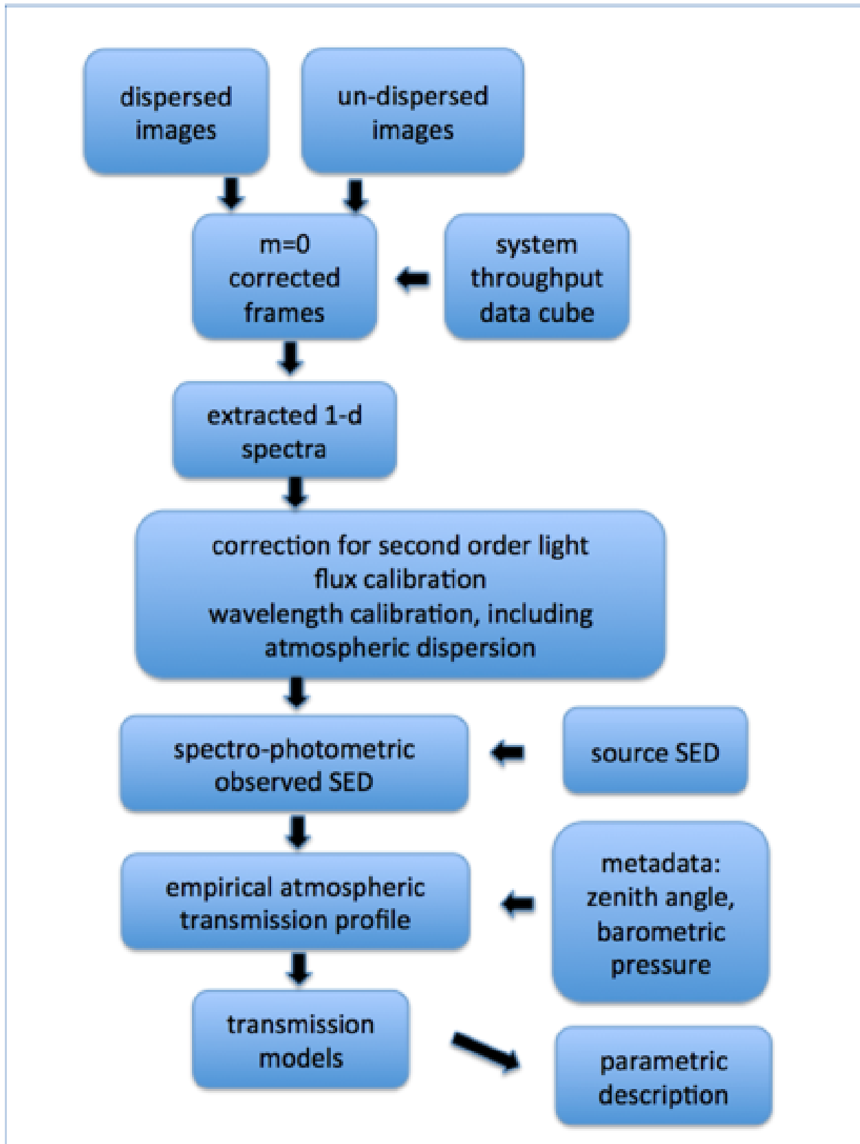
FIGURE 7. Flowchart depicting the atmospheric absorption measurement pipeline, the Rubin Observatory DM Change Control Board. – DRAFT NOT YET APPROVED
