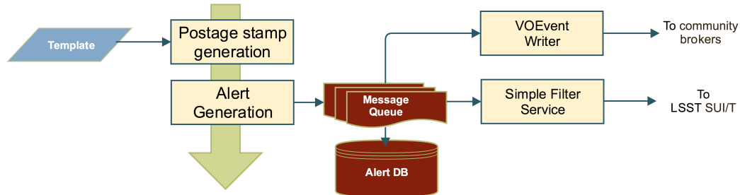
FIGURE 4: Distribution of alerts from the nightly processing: generation of postage stamps around each detected DIAObject, distribution of the DIAObjects as VOEvents, simple filtering of the event stream, and persistence of the events in a database.
