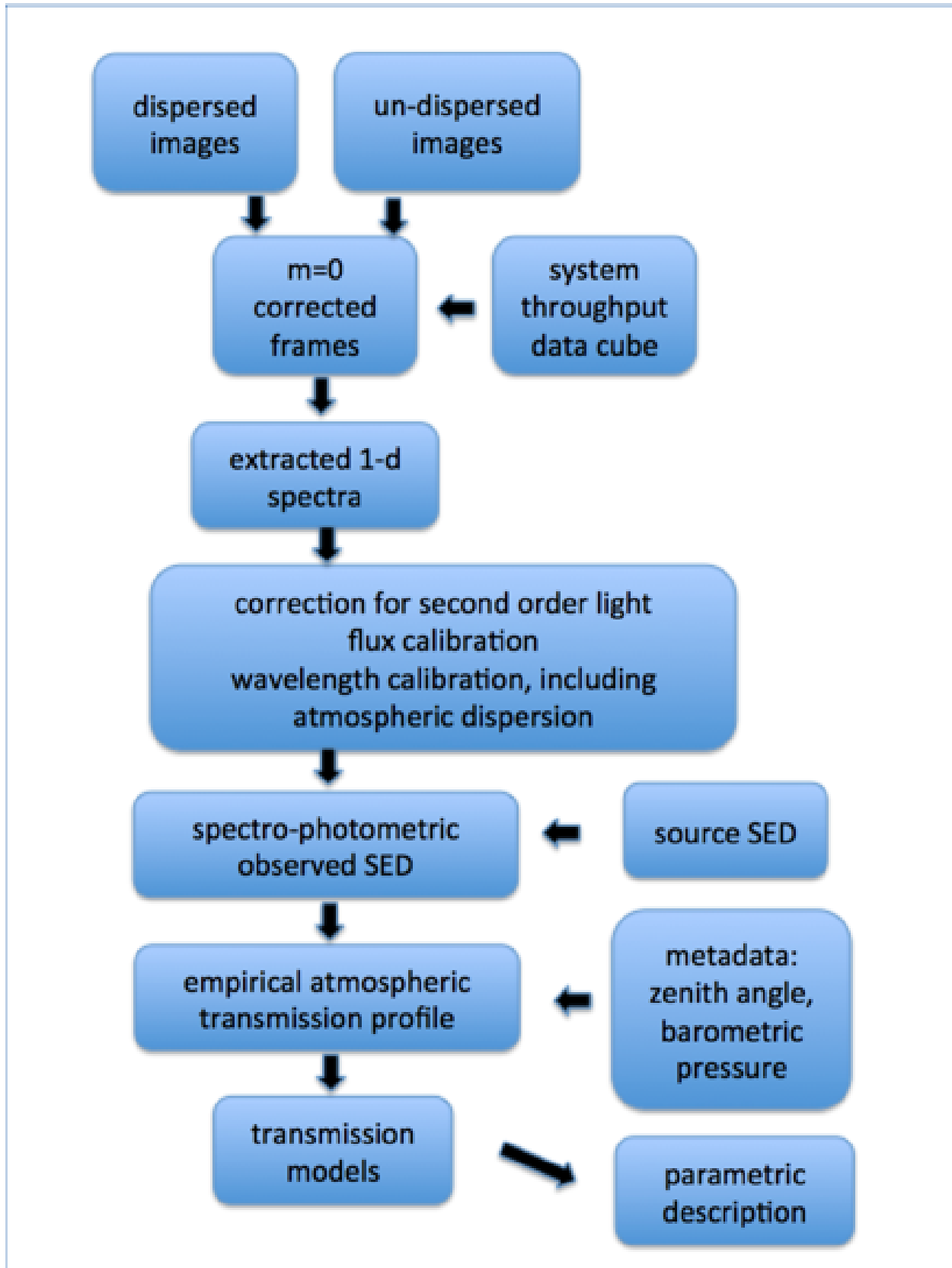
FIGURE 7: Flowchart depicting the atmospheric absorption measurement pipeline. The contents of this document are subject to change without notice by the Rubin Observatory Data Management Science Control Board.
