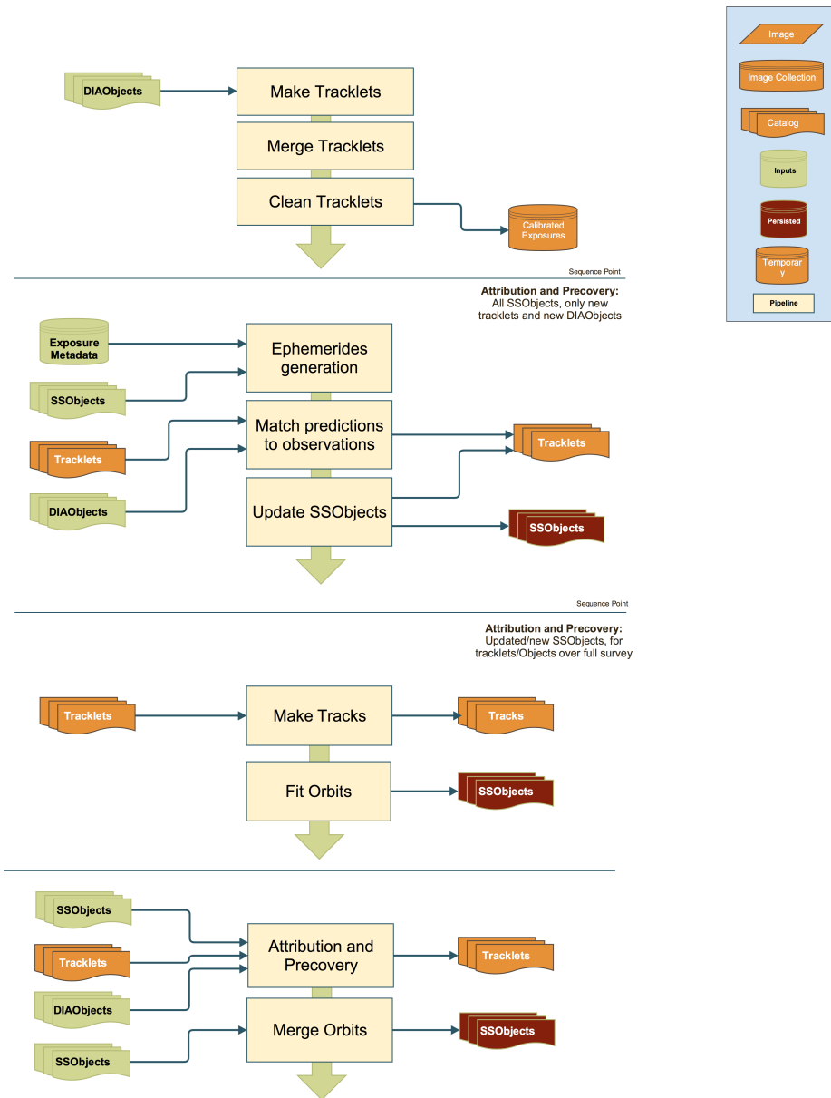
Figure 8: Detection and orbital modelling of moving sources within the nightly data: Tracklet generation from revisits, filtering of tracklets based on known SSObjects , fitting of tracks and orbits to tracklets, pruning of tracklets and DIAObjects based on new and updated SSObjects .
