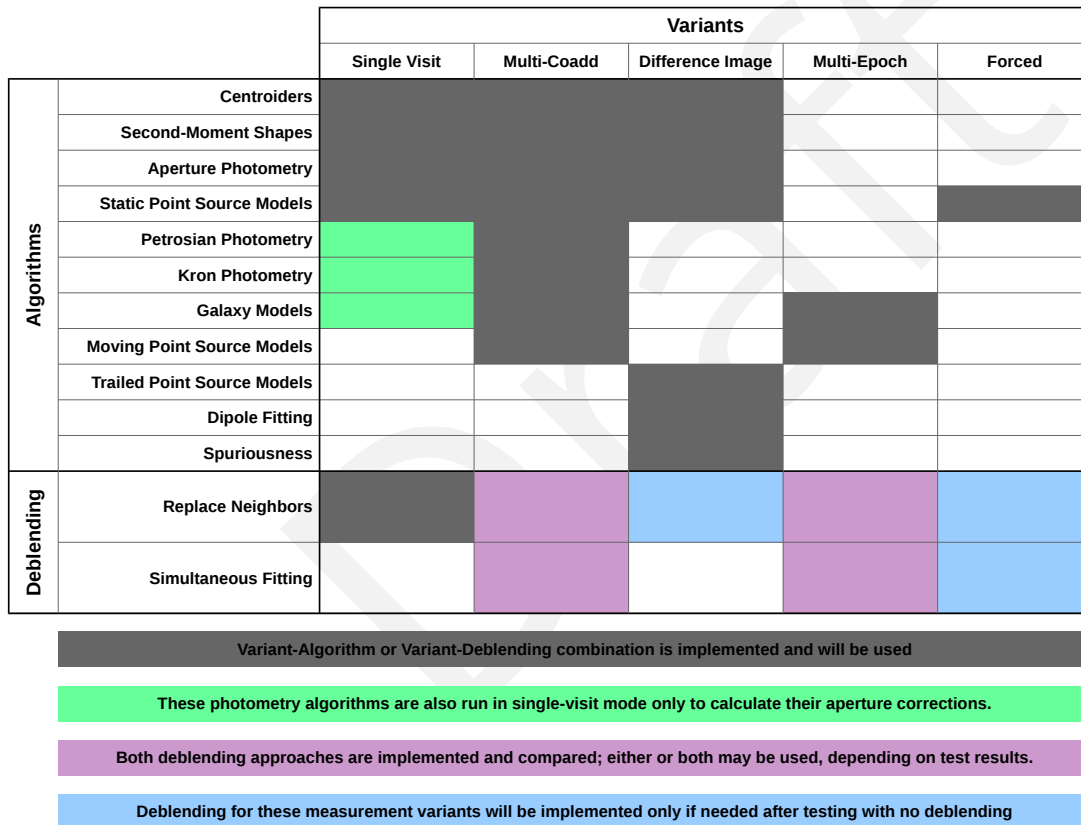
FIGURE 12: Matrix showing combinations of measurement variants, algorithms, and deblending approaches that will be implemented.
