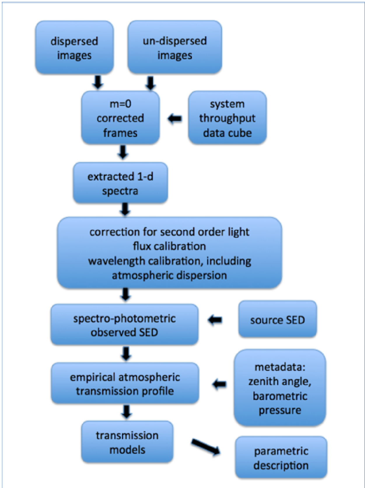
DRAFT NOT YET APPROVED Figure 7.1.1. Flowchart depicting the atmospheric absorption measurement pipeline, the LSST DM Change Control Board. - DRAFT NOT YET APPROVED
