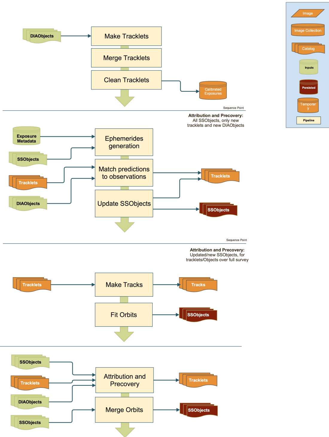
FIGURE 8: Detection and orbital modelling of moving sources within the nightly data: Tracklet generation from revisits, filtering of tracklets based on known SObjects, fitting of tracks and orbits to tracklets, pruning of tracklets and DIAObjects based on new and updated SObjects.
