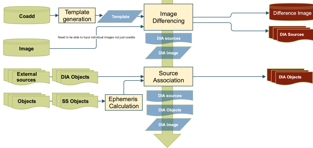
FIGURE 3: Generation of alerts from the nightly data: image differencing and measurement of the properties of the DIASources, identification and filtering of spurious events, association of previously detected DIAObjects and SSObjects with the newly detected DIASources.
