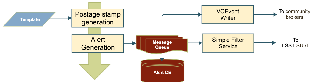
FIGURE 4: Distribution of alerts from the nightly processing: generation of postage stamps around each detected DIAObject, distribution of the DIAObjects as VOEvents, simple filtering of the event stream, and persistence of the events in a database.
