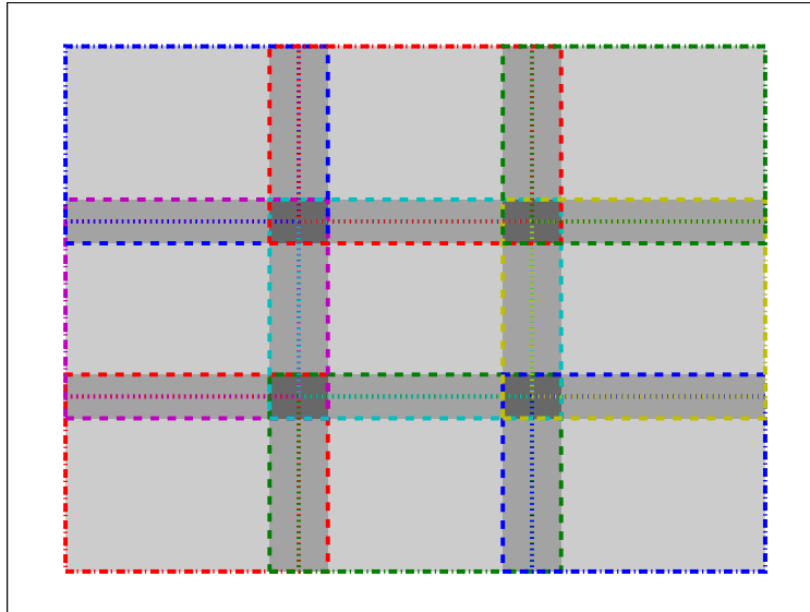
FIGURE 10: Patch boundaries and overlaps regions for a single tract with 3x3 patches. Different colors represent different patches; dashed lines show outer patch regions and dotted lines show inner patch regions. Light gray regions are processed as part of only one patch, medium regions as part of two, and dark regions as part of four.
