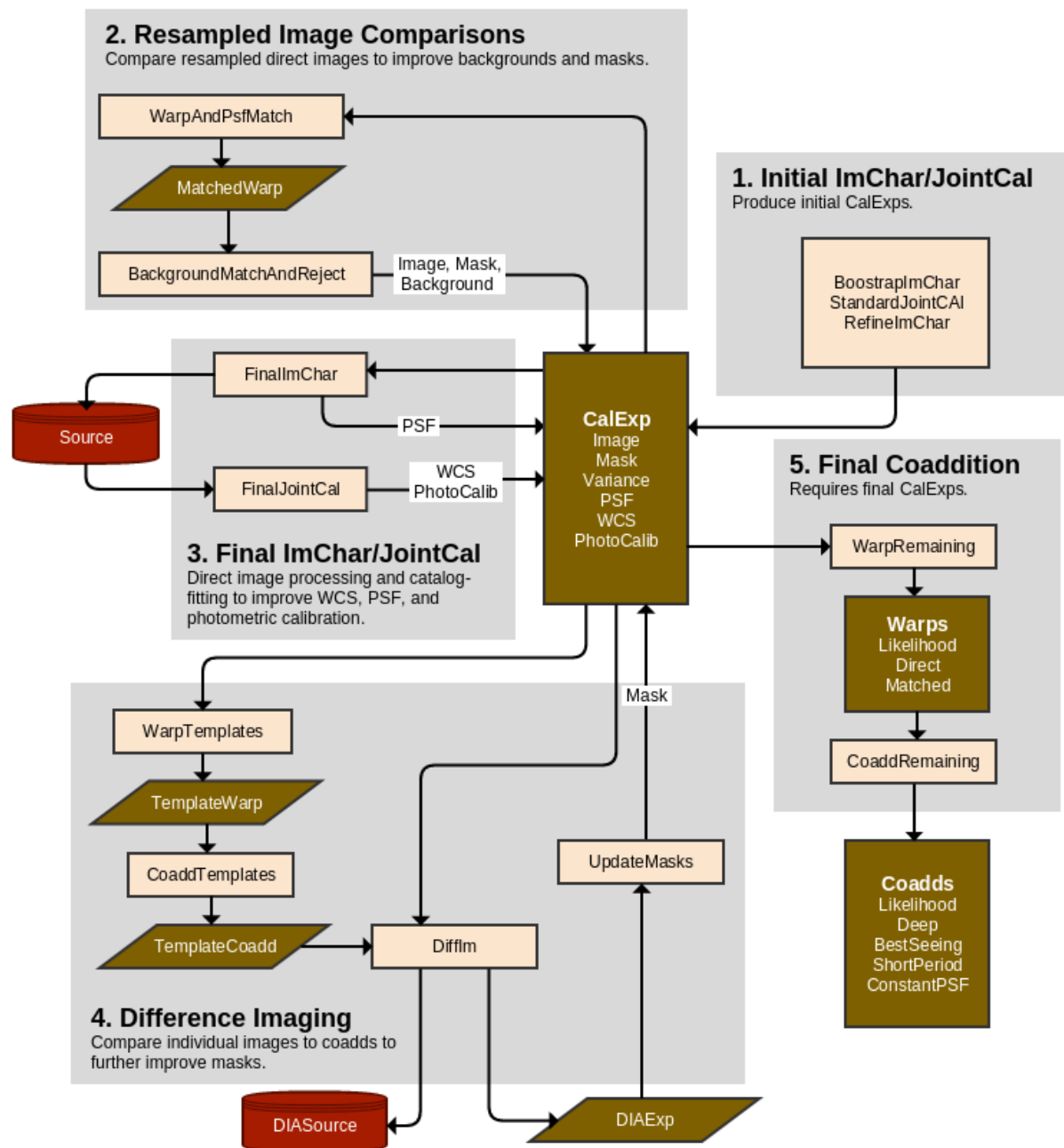
FIGURE 9: Data flow diagram for the Data Release Production image coaddition and image differencing pipelines. Processing proceeds roughly counterclockwise, starting from the upper right with pipelines described in Section 5.1. Each update to a component of the central CalExp dataset can in theory trigger another iteration of a previous loop, but in practice we will “unroll” these loops before production begins, yielding an acyclic graph with a series of incrementally updated CalExp datasets. The nature of this unrolling and the number of iterations will be determined by future algorithmic research. Numbered steps above are described more fully in the text.
