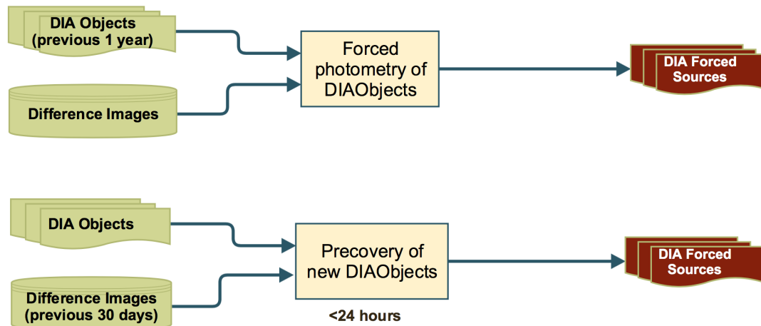
FIGURE 5: Forced photometry for DIAObjects: forced photometry on a night's DiffExp for all DIAObjects that have detected DIASources within the last year, precovery photometry for the previous 30 days of DiffExps for new DIAObjects
