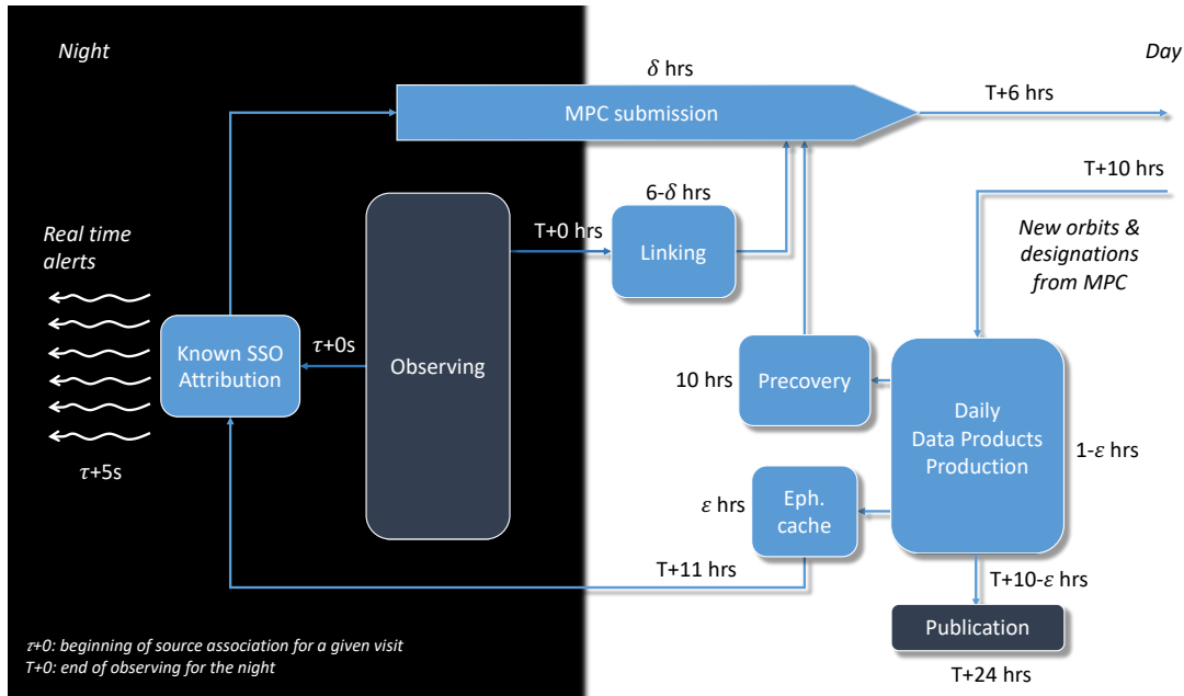
FIGURE 6: Detection, attribution, linking, submission and precovery of moving sources within the nightly data: The attribution is performed in real-time by the attribution service with resulting information attached to the alerts and queued for submission to the MPC. The linking is performed in daytime, with resulting links queued for submission to the MPC. Fetching of data from the MPC is performed at least once daily, triggering recomputation of physical properties and precovery runs. Any observations discovered by the precovery procedure are queued for submission to the MPC. The ephemeris cache is precomputed after the daily fetch of orbit information from the MPC, to enable fast attribution at nighttime. All timings denote design goals.
